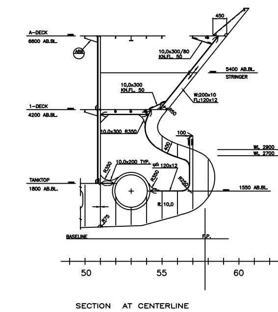
SECTION AT CENTERLINE
