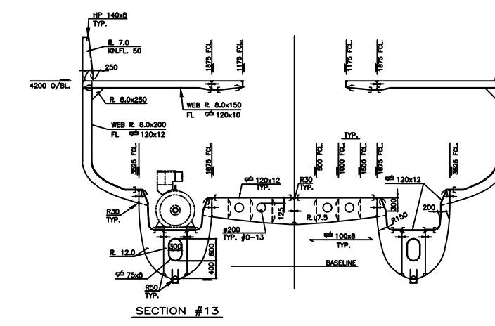
SECTION #13
