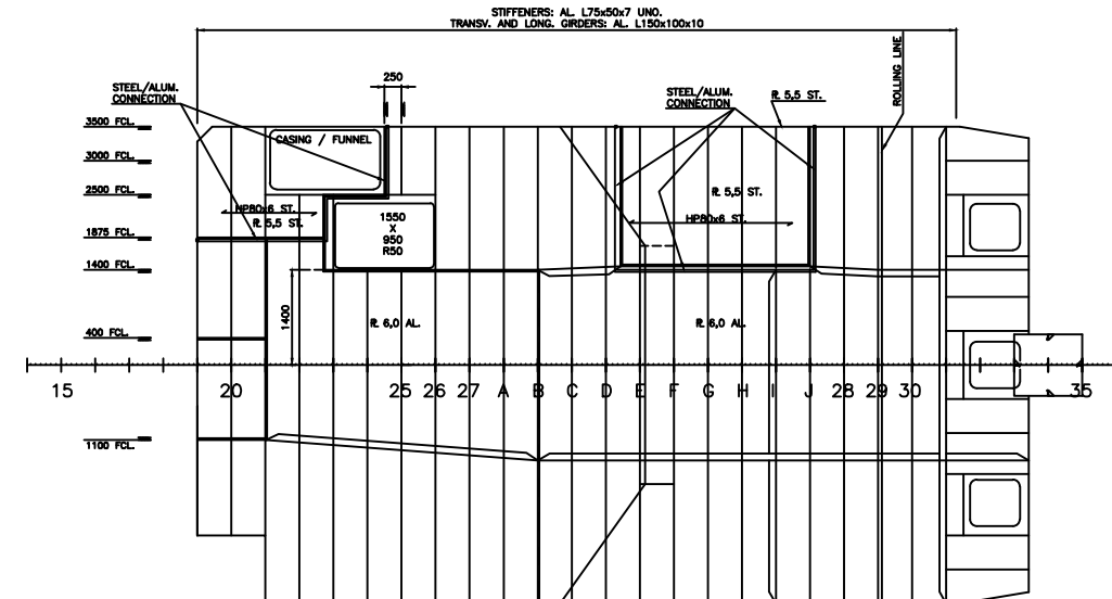
WHEELHOUSE FLOOR / SUPERSTRUCTURE TOP 8000 AB.B.
